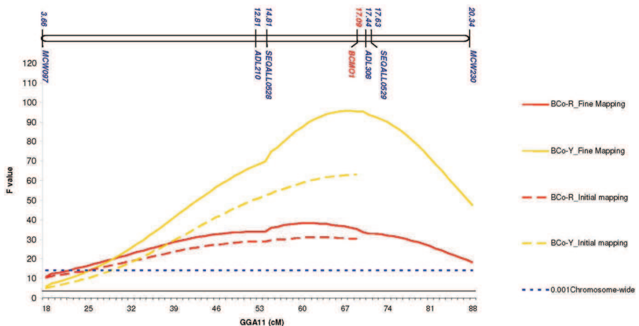
Figure 1. Relative position of the yellowness (BCo-Y) and redness (BCo-R) QTL and of the BCMO1 gene. F profiles show a better localization of the BCo-Y and BCo-R trait QTL by genetic map densification (solid lines) with six markers compared to initial mapping (dashed lines) with three markers (MCW097, ADL210 and ADL308). BCMO1 gene is located on GGA11 between 17.085 and 17.105 Mbp, the approximate location of the observed BCo-Y QTL.
