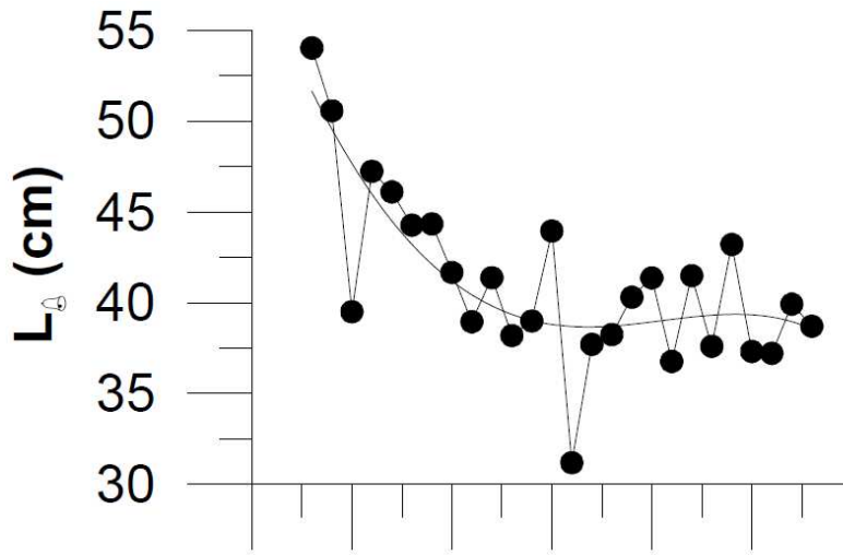
Figure A2.6. Time-series of the Mean maximum length indicator (MMLI) applied to the IBTS Q1 groundfish survey data from 1983 (the start of consistent Q1 IBTS) up to 2008. At its lowest point in 2001, the indicator fell to a value for the Kattegat and Skagerrak. Results based on (ICES 2009).
