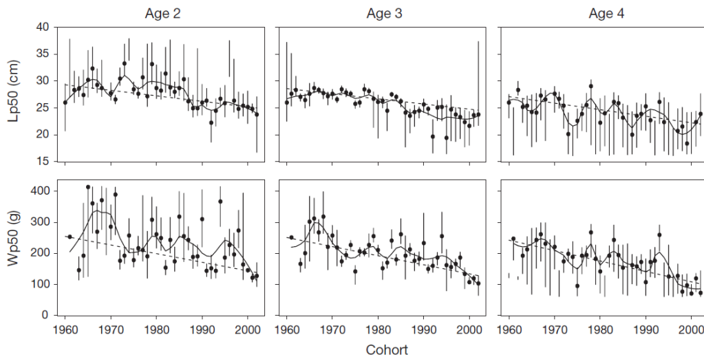
Fig. 4.17. PMRNI for North Sea sole ( Solea vulgaris ) reaction norm midpoints L_{p50} and W_{p50} over time (dots), bootstrapped 95% percentiles (vertical bars), trend regression weighted by the inverse bootstrap variances (---) and fit with a non-parametric smoother. All trends are significant on a level of \alpha = 10^{-4}
