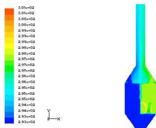
Fig. 8. Temperature field, heat source 6kW, inlet velocity 4 \text{ m/s} , opening 50%-50%.
