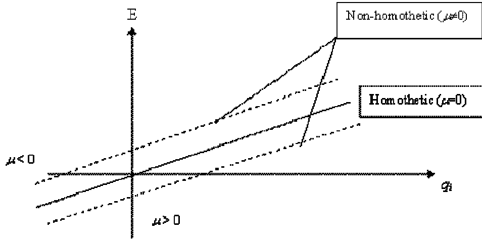
Figure 1: Engel curves
