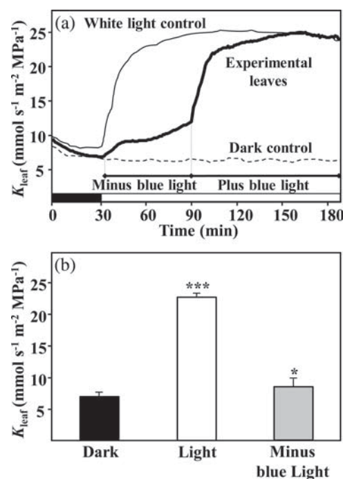
Figure 6. (a) Typical time courses of leaf hydraulic conductance ( K_{leaf} ) response of J. regia under white light and dark conditions (control mean), and under filtering for blue light wavelengths (minus blue light) followed by a return to ambient full spectrum white light condition (plus blue light) (experimental leaves). Leaf hydraulic conductance data were recorded using an HPFM method. Black bar on the x-axis corresponds to the dark periods. (b) Mean K_{leaf} values ( \pm SE) in control dark, control light, and minus blue light leaves. Asterisks represent significant differences (Student's t ) (* 0.01 < P < 0.05 ; *** P < 0.001 ).
