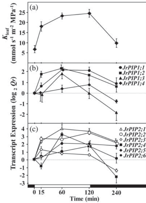
Figure 5. Time courses of leaf hydraulic conductance response ( K_{leaf} ) (a) and kinetic changes in transcript expression ( \log_2 Q_r ) of JrPIP1 s (b) and JrPIP2 s (c) in leaves of J. regia under conditions of light (white bar) and darkness (black bar). Leaf hydraulic conductance data were recorded using an HPFM method. Relative transcript expressions were determined by real-time quantitative RT-PCR using PIP1 or PIP2 specific primer sets for each isoform. Dark leaves were used as controls for relative expression calculations, and 18S rRNA gene expression was used as endogenous control. Expression levels ( \log_2 ) are presented as expression ratio (treated to dark control). Black and white bars on the x-axis correspond to the dark and light periods, respectively. Data correspond to means of three technical repeats from three independent biological experiments, and bars represent standard error ( n = 9 ).
