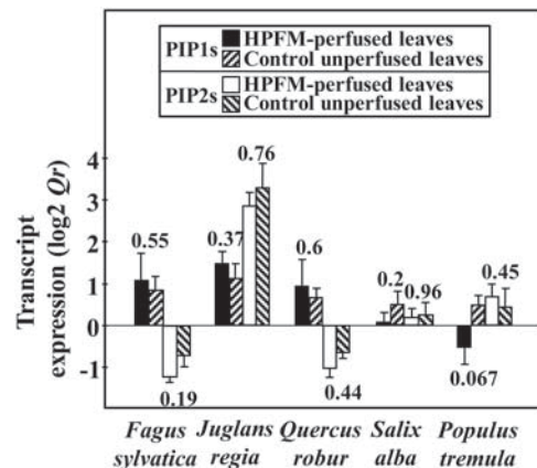
Figure 3. Comparison of transcript expression changes of PIP1 and PIP2 aquaporin groups for five tree species in dark condition and after 2 h white light exposure in HPFM water-perfused and control-unperfused leaves. Dark leaves were used as controls for relative expression calculations. The 18S rRNA gene expression was used as endogenous control. Expression levels ( \log_2 ) are presented as expression ratio (treated to dark control). Relative transcript expressions were determined by real-time quantitative RT-PCR using generic PIP1 or PIP2 primer sets designed within conserved regions between selected species. Numbers represent Student's t -test P values for average HPFM-perfused expression versus control-unperfused levels (no difference in expression if P < 0.05 ).
