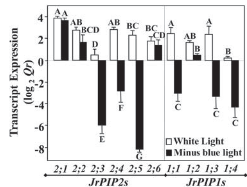
Figure 7. Changes in transcript levels of the JrPIP1 s and JrPIP2 s in leaves of J. regia after 2 h exposure to white light or with blue light wavelengths filtered out (minus blue light). Dark leaves were used as controls for relative expression calculations. The 18S rRNA gene expression was used as endogenous control. Expression levels ( \log_2 ) are presented as expression ratio (treated to dark control). Relative transcript expression of indicated genes was determined by real-time quantitative RT-PCR using specific primer sets for each isoform. Data correspond to means of three technical repeats from three independent biological experiments, and bars represent standard error ( n = 9 ). Levels not connected by same letters are significantly different (Tukey HSD).
