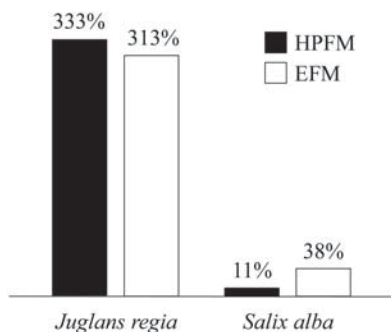
Figure 2. Methodological comparison of HPFM and EFM for measuring K_{leaf} after 2 h under high irradiance (%) relative to dark control in J. regia and S. alba ( n = 5 ).
