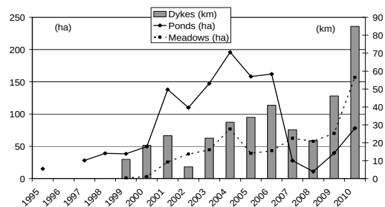
Figure 3. Progressive colonization of different habitats in Brière.
