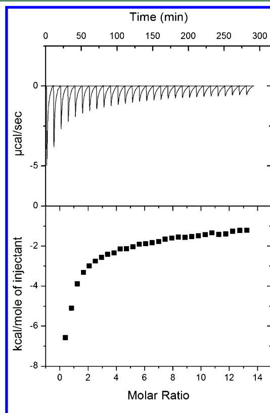
Figure 1. Microcalorimetric titration of \beta lg with linoleate in PBS buffer (pH 7.4) at 60 °C. (A) raw heat signal for the titration of \beta lg (0.16 mM) with 10 \mu L increments of 9.64 mM linoleate. (B) Area under each peak integrated and plotted against the linoleate/ \beta lg molar ratio.
