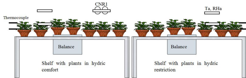
Fig. 1. Experimental device.
