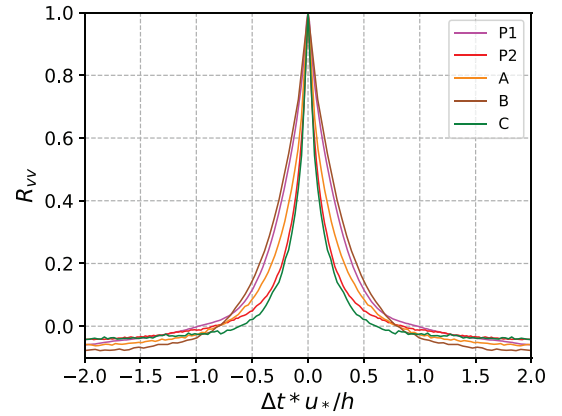
Fig. 21 Correlation coefficient of the spanwise velocity component R_{vv} at z = h/2
