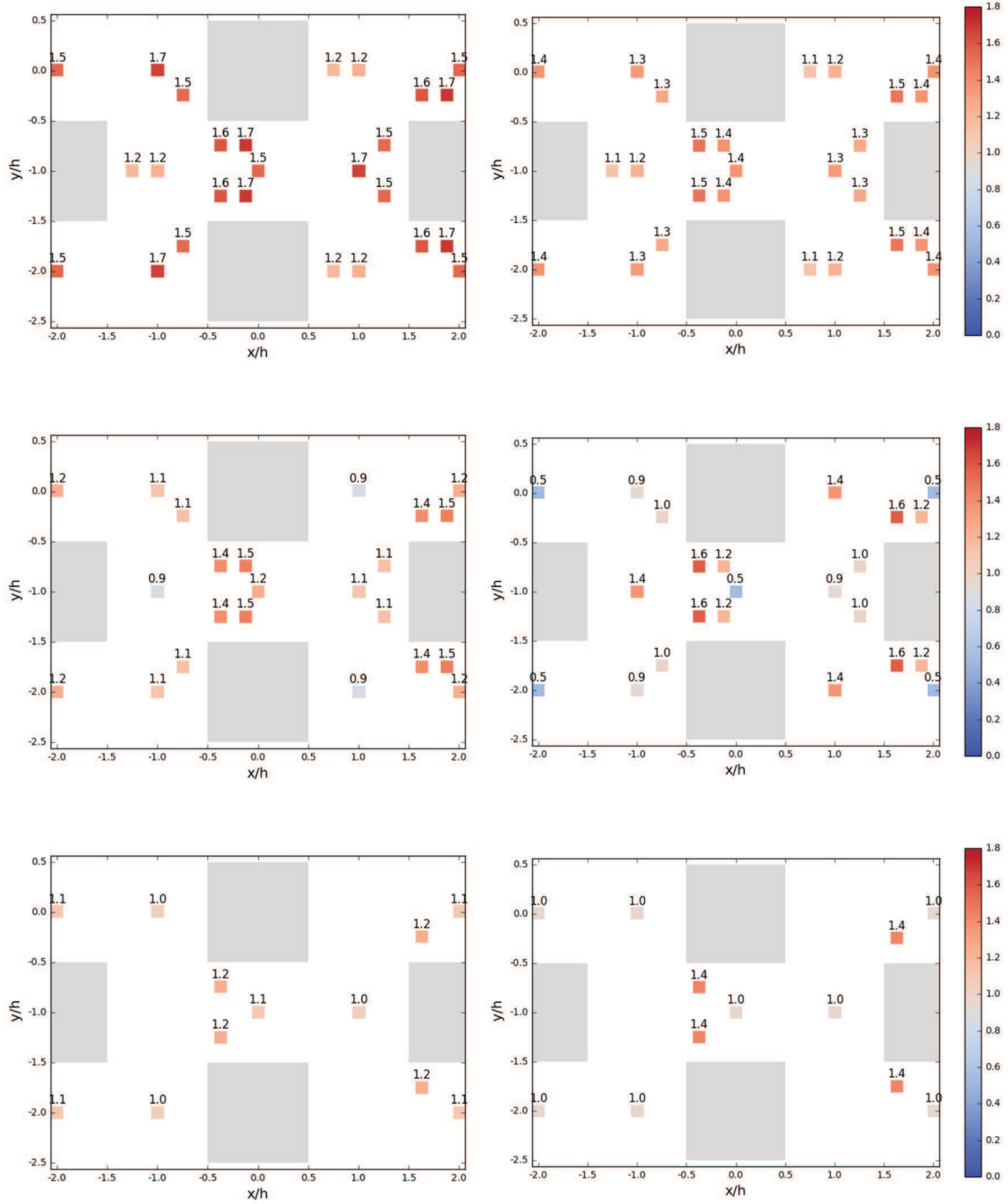
Fig. 7 Maps of standard deviation of streamwise velocity u_{\text{RMS}}/u_* (left column) and standard deviation of spanwise velocity v_{\text{RMS}}/u_* (right column) in wall-parallel planes inside the canopy at various
