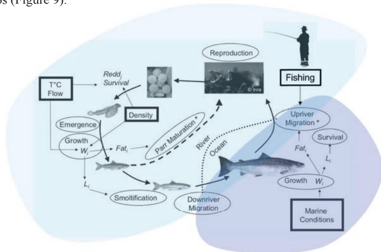
Figure 9: Schematic of an Individual Based Atlantic Salmon model (IBASAM), that allows simulation of the response of salmon to climate change scenarios.
