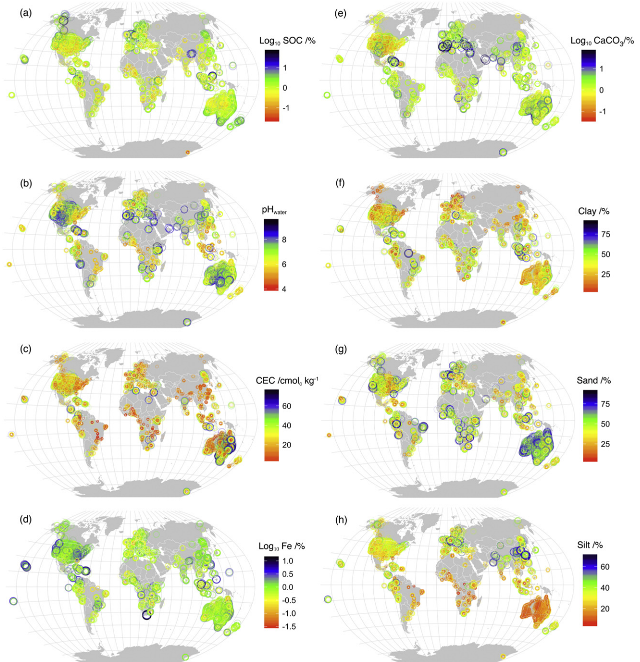
Fig. 11. Spatial distribution of the predicted soil attribute data harmonised with the spectroscopic method. The attributes shown are (a) soil organic C (SOC) in the log scale, (b) \text{pH}_{\text{water}} , (c) cation exchange capacity (CEC), (d) extractable Fe in the log scale, (e) soil inorganic C (SIC) in the log scale, (f) clay content, (g) sand content and (h) silt content. For (a), (d) and (e) we transformed the predictions to the log scale to help visualise their global variability. Circles are proportional to concentration and when there is more than one measurement per site (i.e. measurements at different depths), they overlap.
