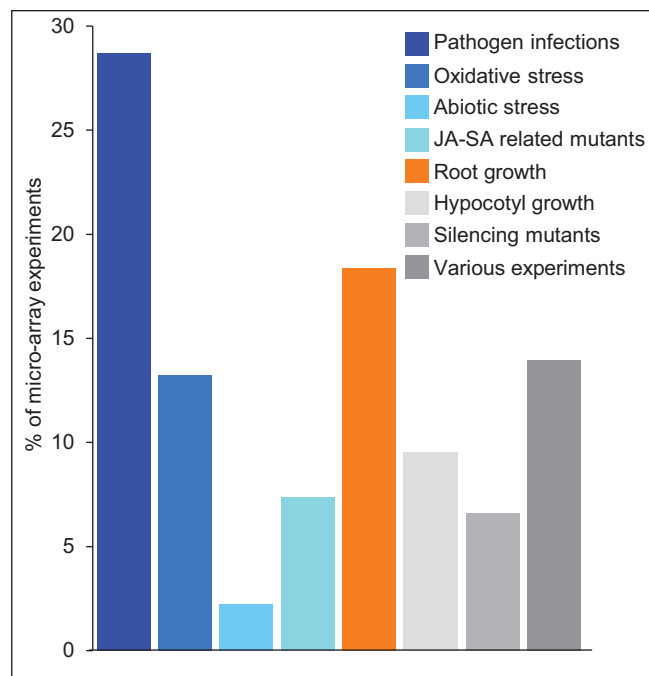
Fig. 1. Synthesis of the results from the 136 experiments in which AT5G44585 was significantly deregulated (Bonferroni P -value < 5\% ) within the CATdb resource, then sorted into eight classes: pathogen infections, oxidative stress, abiotic stresses, JA-SA-related mutants, root growth, hypocotyl growth, silencing mutants, and various experiments. The whole set of results is detailed in Supplementary Table S2.
