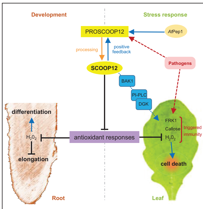
Fig. 11. Putative model explaining the SCOOP12 functions in root development and biotic stress response through the inhibition of protection against oxidative stress. The red dotted arrows represent the action of the pathogens; the induction and the repression effects are represented by blue and black lines, respectively. PI-PLC, phosphatidylinositol-specific phospholipase C; DGK, diacylglycerol kinase.
