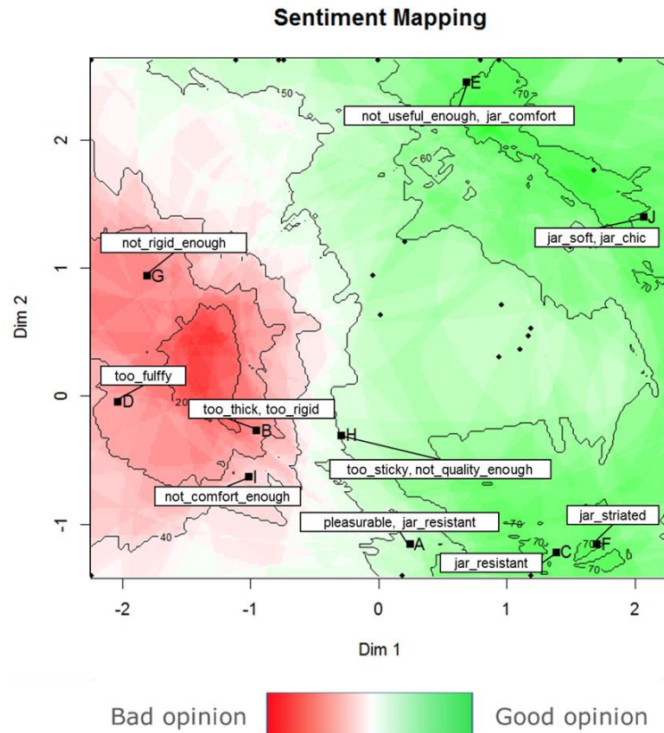
Figure 8: Sentiment Mapping provided thanks to the car seat leatherette dataset
