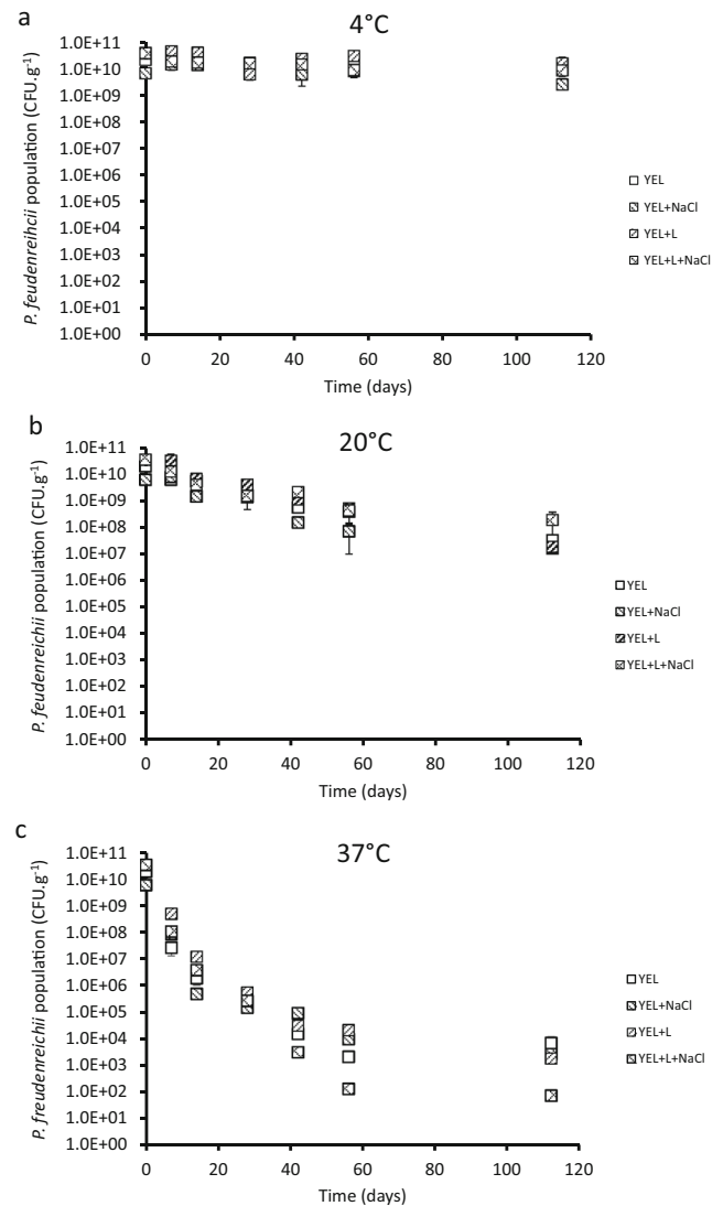
Fig. 5 Storage temperature and P. freudenreichii adaptation modulates its viability during powder storage. The different powders were stored at 4 °C (a), 20 °C (b), and 37 °C (c) for 115 days. P. freudenreichii populations in spray-dried powders were quantified by CFU counting (as described in the “Material and methods” section) during storage. YEL: yeast extract lactate. L: lactose
