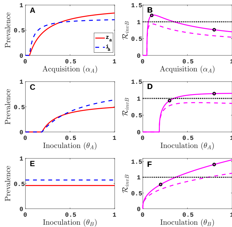
Figure 2. For the vector-explicit model, the virus A equilibrium prevalences for the vector z_a = za_{eq}/\bar{V} and for the host i_a = ia_{eq}/\bar{P} are graphed in panels (A,C,E) and the corresponding invasion reproduction numbers \mathcal{R}_{invB} are graphed in panels (B,D,F) as a function of acquisition ( \alpha_A ) or inoculation ( \theta_A and \theta_B ) parameters. Virus B may invade the virus A equilibrium if the invasion reproduction number is greater than the threshold value one. The parameters values that are not varied are fixed at their default values (see Table 2): \Lambda = 10 per month per unit area, \Phi = 30 per month, c = 1 per month, \alpha_A = 0.2 , \alpha_B = 0 , \alpha_{AB} = 0.5 , \epsilon_A = \epsilon_B = 0.5 , \delta_A = \delta_B = 3 per month, \mu = 1/12 per month, \sigma = 1000\mu (1000 per year per unit area), \theta_A = 0.8 , \theta_B = 0.5 and \omega = \omega_A = \omega_B = 0 . Parameter values for the two invasion reproduction curves in (B,E,F) are \gamma_B = 0.9 for the solid curve and \gamma_B = 0.25 for the dashed curve. (B) The two black circles on the solid curve are at values of \alpha_A = 0.1, 0.8 ; (D) \theta_A = 0.3, 0.8 ; (F) \theta_B = 0.2, 0.8 . The invasion reproduction number is \mathcal{R}_{invB} = \rho(M_{invB}) as defined in (5).
