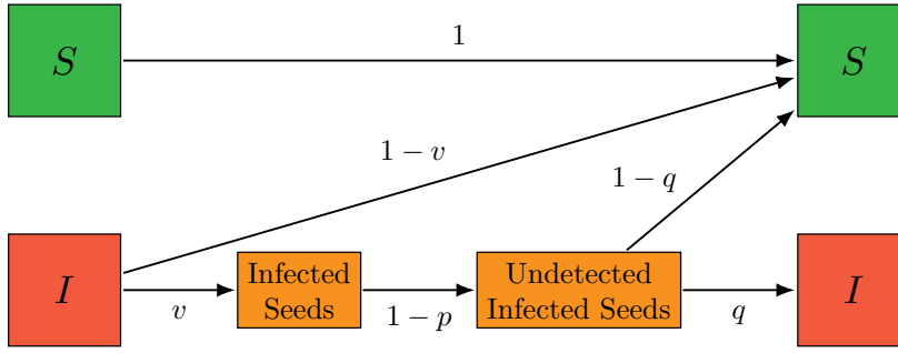
Fig. 1 Replanting dynamics as expressed in Equation 1. The arrows represent the possible pathways that seeds can take from the compartments on the left to the compartments on the right. The parameters next to each arrow represent the probabilities that seeds move along that pathway.
