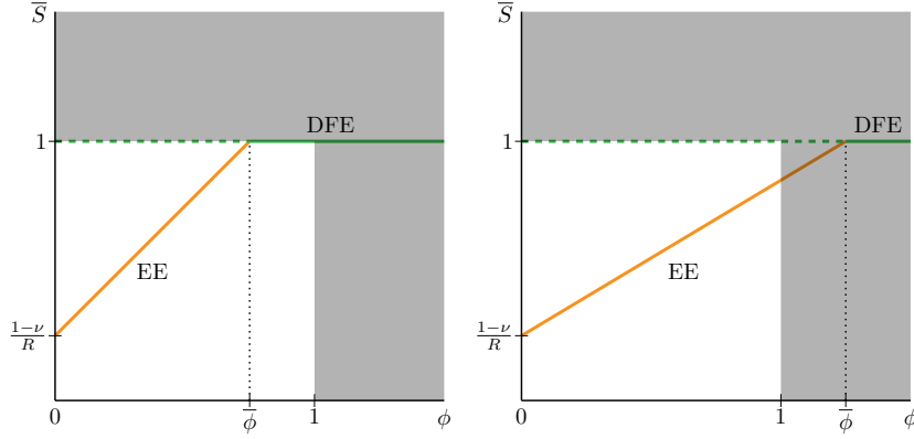
Fig. 2 Dynamics of the S-I disease model. \bar{\phi} = 1 - \frac{1-\nu}{R} . DFE means Disease free equilibrium, EE means endemic equilibrium. The biologically feasible region is in white. (Left) Case (B): Dynamics for the case R < 1 . (Right) Case (A): Dynamics for the case R > 1 .
