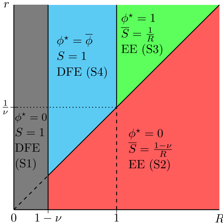
Fig. 4 Results of static optimization: The (R, r) plane is divided into distinct regions with differing control strategies.
