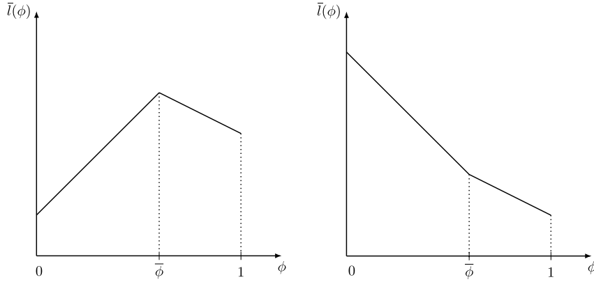
Fig. 3 Long term payoff as a function of \phi in the case (B) R < 1 . (Left) Case B1: the maximum occurs at \phi = \bar{\phi} . (Right) Case B2: the maximum occurs at \phi = 0 .
