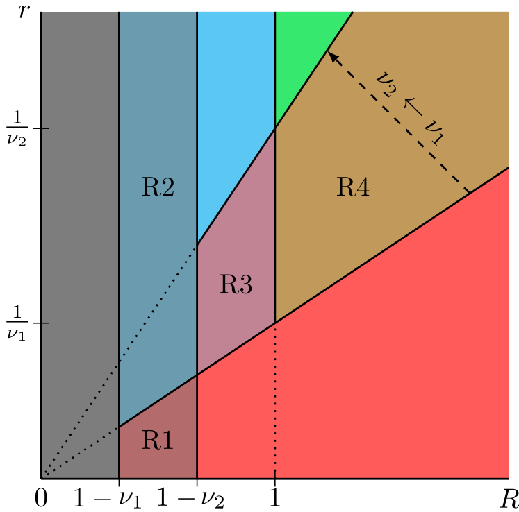
Fig. 5 Changes to the (R, r) plane as \nu varies: Decreasing the value of \nu from \nu_1 to \nu_2 results in 4 regions where the control strategy has changed.
