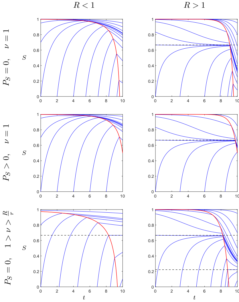
Fig. 6 Dynamics of different combinations of R , P_S , and \nu . Blue curves are trajectories under optimal control, Red curve is the switching curve, and dashed lines are equilibrium values for \phi = 0 and \phi = 1 when they differ from \bar{S} = 0 and \bar{S} = 1 respectively. (Left Panel) R < 1 : \sigma = 1 , \beta = \frac{1}{2} , p_S = 3 , c = 1 , \nu \in \{1, \frac{2}{3}\} , P_S \in \{0, 2\} , (Right Panel) R > 1 : \sigma = 1 , \beta = \frac{3}{2} , p_S = 3 , c = 1 , \nu \in \{1, \frac{2}{3}\} , P_S \in \{0, 2\} .
