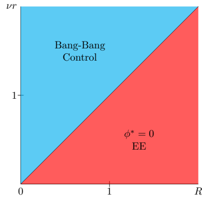
Fig. 7 Results of dynamic optimization: The (R, \nu r) plane is divided into distinct regions with differing control strategies. Examples of this bang-bang control can be seen in Figure 6.
