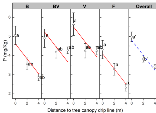
Fig. 2. Available Phosphorus (P) mean changes by the distance of the olive tree row according to intercrop ( Vicia sativa L., V; Hordeum vulgare L., B; mixture of 40% Hordeum vulgare and 60% Vicia sativa , BV; Fallow, F). Significant at 5% level
