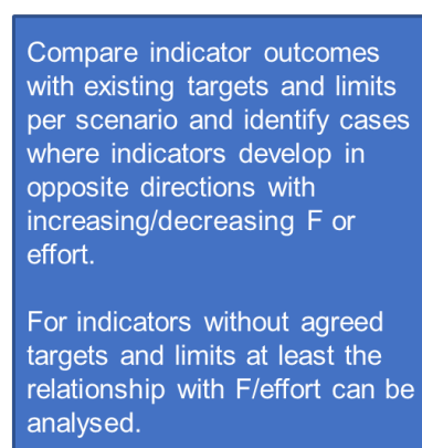
Figure 3.1. General approach to test the consistency of existing targets and limits for indicators in an ecosystem context.
