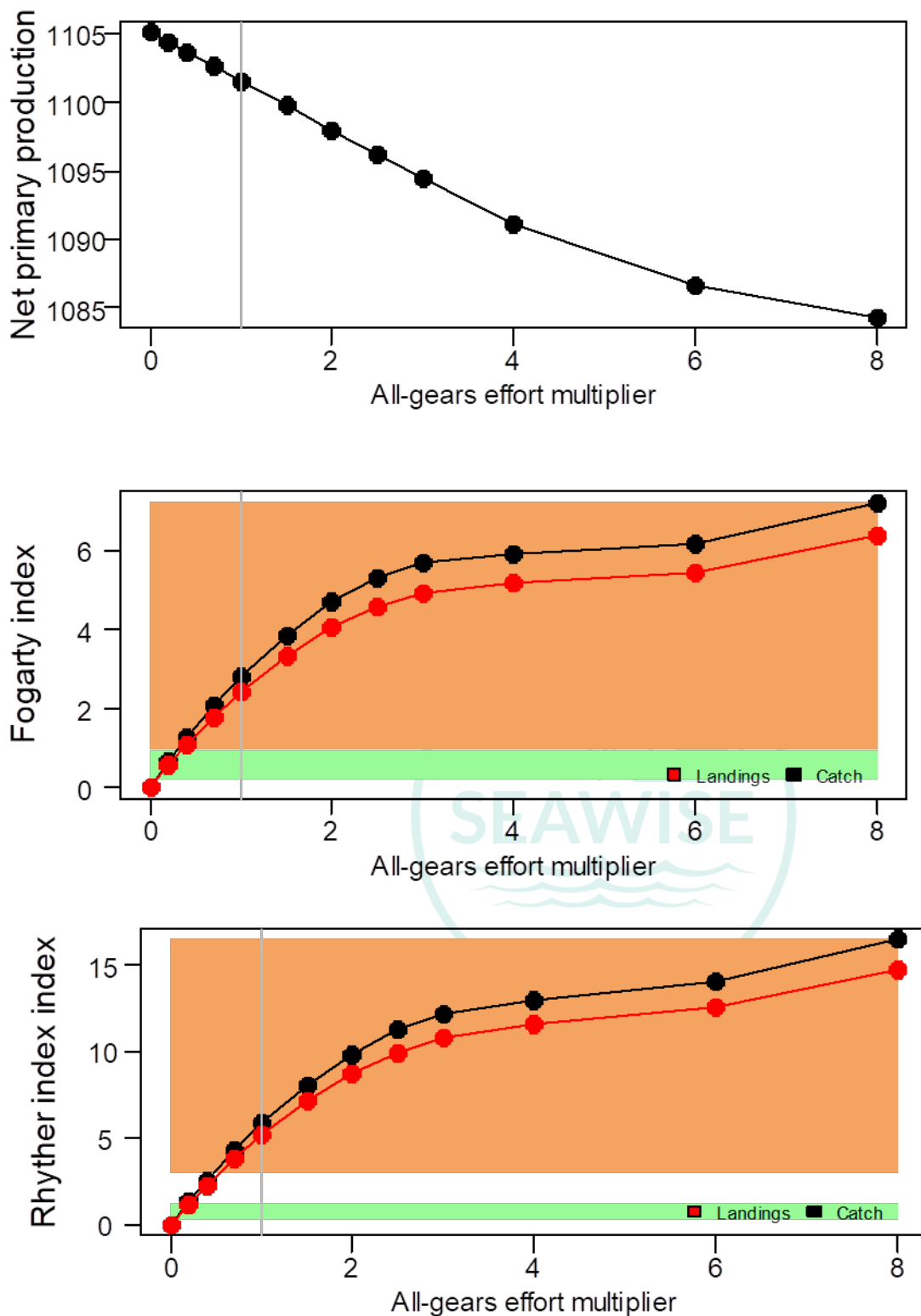
Figure 25. Upper panel: Annual net primary production (mMolesN.m -2 .y -1 ) simulated by the Celtic Sea model in relation to effort multiplier scenarios. Middle panel: Fogarty index (landings or catch divided by net primary production) relative to effort multiplier scenarios. Lower panel: Ryther index (catch or landings tonnes.km -2 .y -1 ) relative to effort multiplier scenarios. Green shaded areas in the Fogarty index and Ryther index panels are regarded as optimal ranges (Link & Watson 2019; Beet & Gaichas 2022). The orange shaded areas are regarded as representing ecosystem overfishing. Vertical grey line at effort multiplier = 1 in each panel represents the baseline 2003-2013 model.
