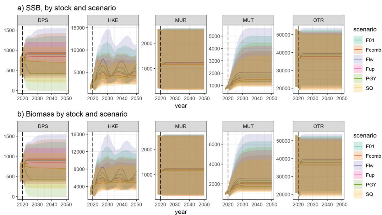
Figure 2. Biological indicators a) Spawning stock biomass (SSB), b) total biomass of the stocks under consideration (DPS, HKE, MUT, MUR, OTR) by scenario in the eastern Ionian Sea. Coloured ranges correspond to 95% intervals from 292 iterations.
