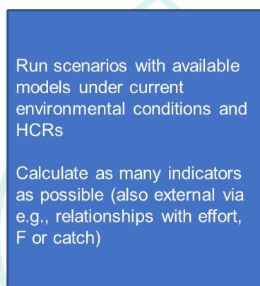
Figure 3.1. General approach to test the consistency of existing targets and limits for indicators in an ecosystem context.
