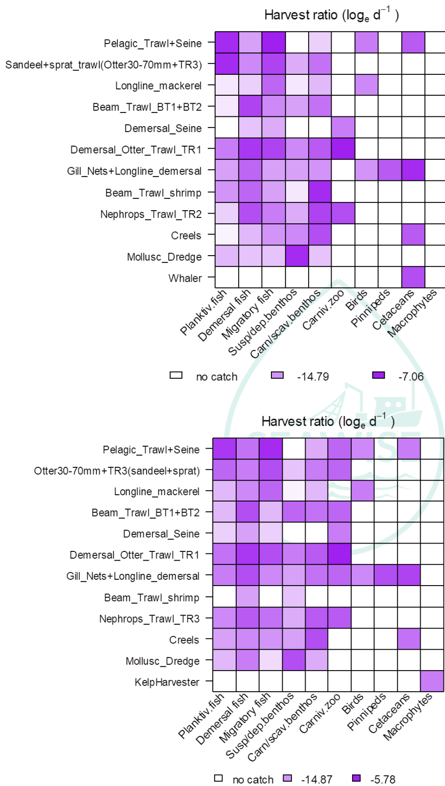
Figure 5. Harvest ratios ( d^{-1} ) by each gear on each guild in the 2003-2013 North Sea (upper panel) and Celtic Sea (lower panel) models.
