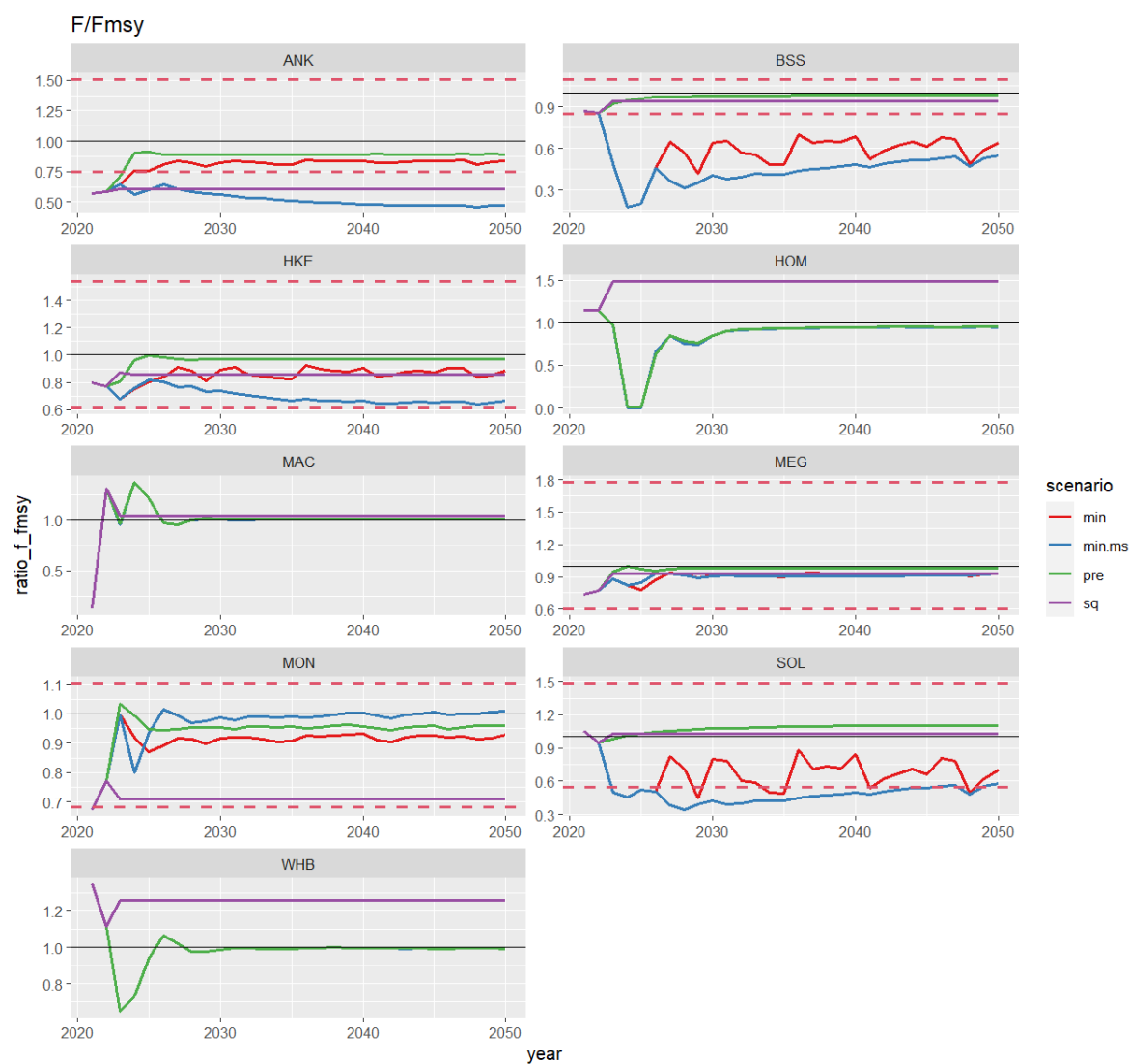
Figure 2. Ratio between fishing mortality and Fmsy time series. For demersal species the horizontal red dashed lines correspond with F_{upp} and F_{low} and for all the stocks the horizontal black line with F_{msy} .
