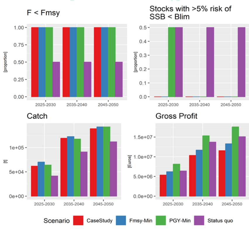
Figure 4.3.1. CFP indicators per scenario and time period predicted by the BEE-FISH model for the Western Baltic
