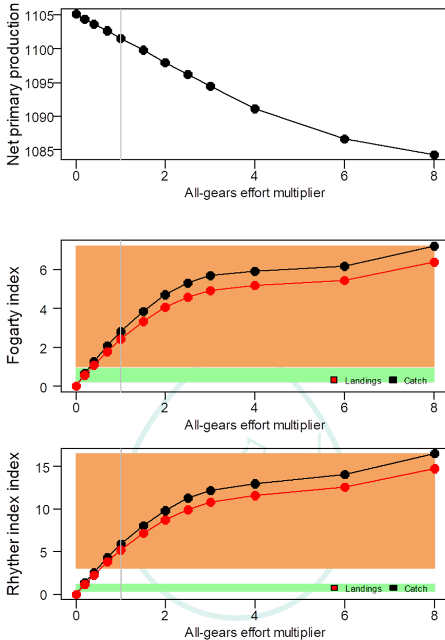
Figure 4.2.8. Upper panel: Annual net primary production ( \text{mMolesN.m}^{-2}.\text{y}^{-1} ) simulated by the Celtic Sea model in relation to effort multiplier scenarios. Middle panel: Fogarty index (landings or catch divided by net primary production) relative to effort multiplier scenarios. Lower panel: Ryther index (catch or landings tonnes. \text{km}^{-2}.\text{y}^{-1} ) relative to effort multiplier scenarios. Green shaded areas in the Fogarty index and Ryther index panels are regarded as optimal ranges (Link & Watson 2019). The orange shaded areas are regarded as representing ecosystem overfishing. Vertical grey line at effort multiplier = 1 in each panel represents the baseline 2003-2013 model.
