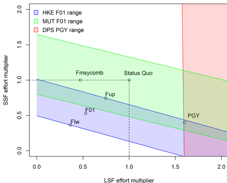
Figure 4.4.1. Effort multipliers by fleet for the six scenarios defined for the eastern Ionian Sea (GSA 20) bioeconomic projections. The coloured areas correspond to fishing mortality ranges of the three main stocks; Fup to Flw range for red mullet (MUT) and hake (HKE) and PGY (fishing mortality corresponding to 80%MSY) for deep water rose shrimp (DPS). The effort multiplier set for the PGY scenario is defined on the intersection of the three species ranges.
